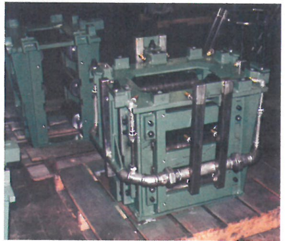
Continuous Caster Foot Roll Assemblies
